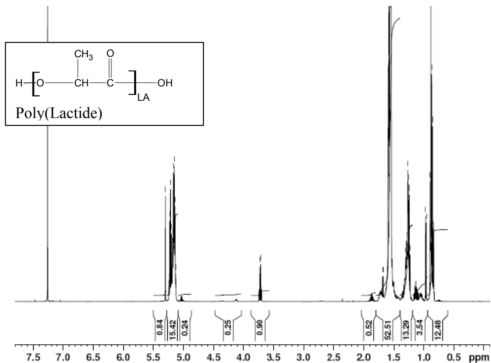
NMR of PLA polymer
